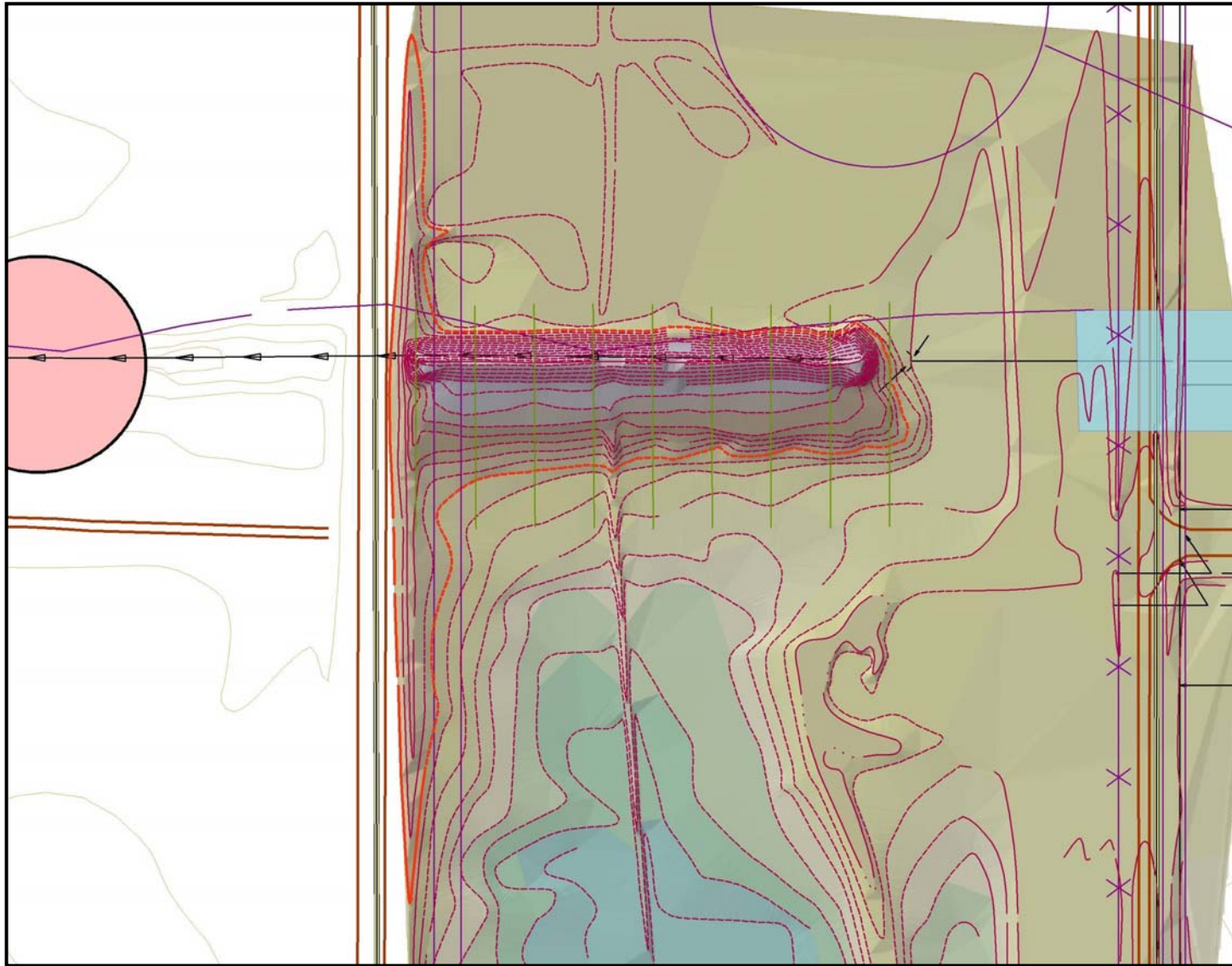
Figure 4. Drop Inlet and Existing Culvert at Outfall 011 Pond
