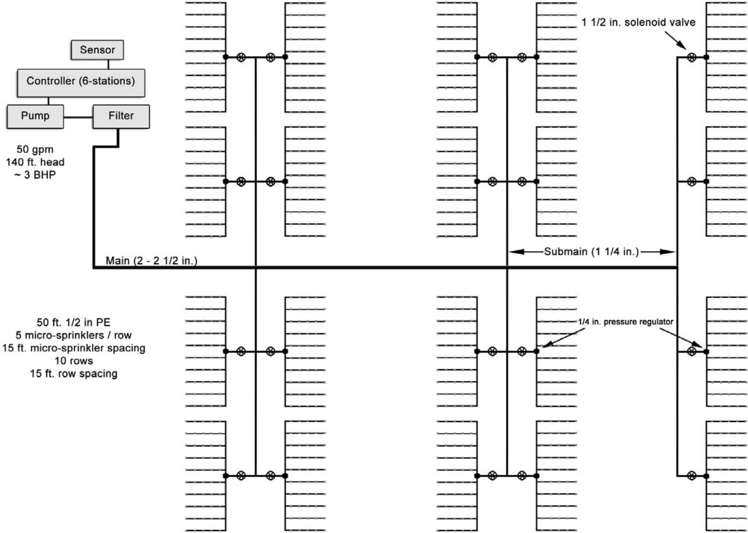
Figure 11. 5-Acre Micro-sprayer Irrigation System Layout
