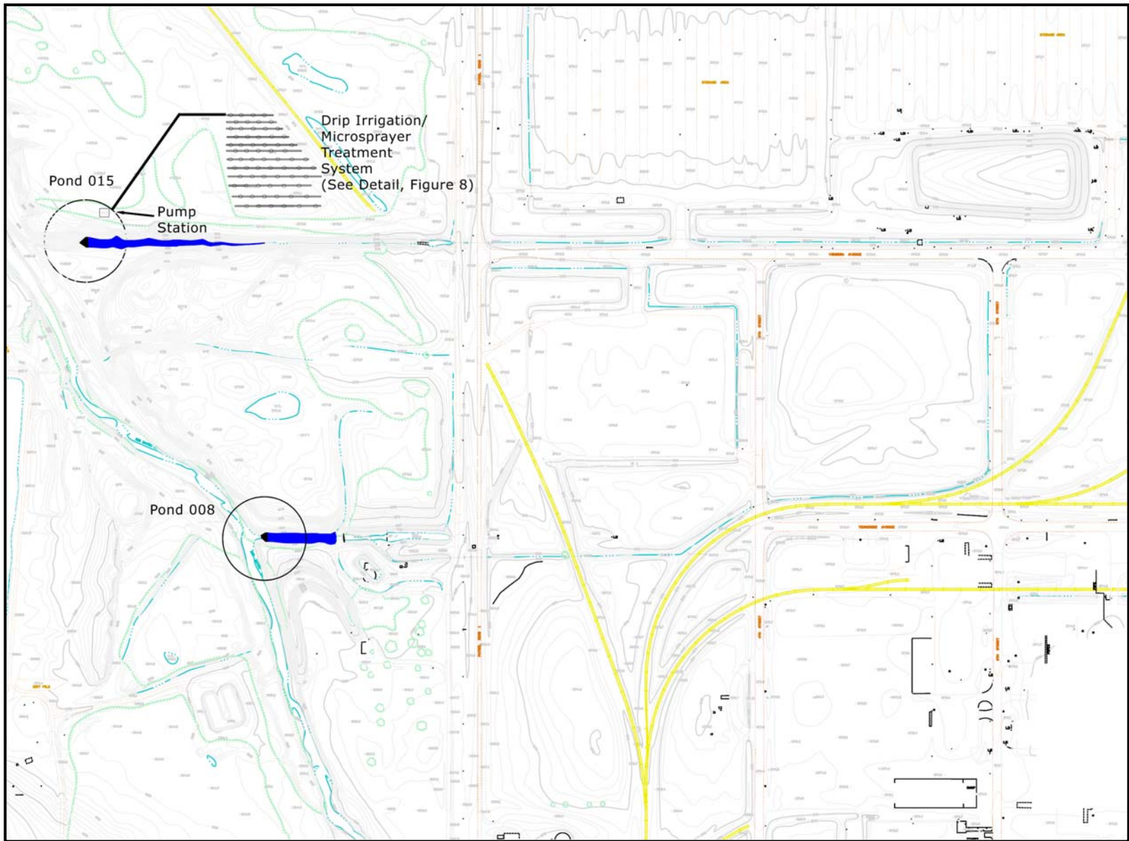
Figure 9. Drip and Micro-sprinkler Irrigation System - Outfall 015
