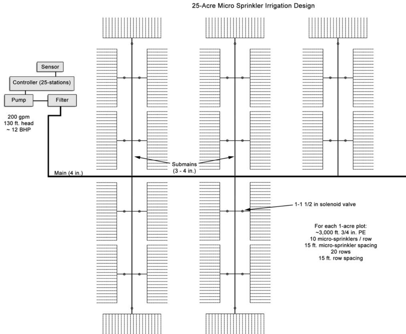
Figure 12. 25-Acre Micro-sprayer Irrigation System Layout
