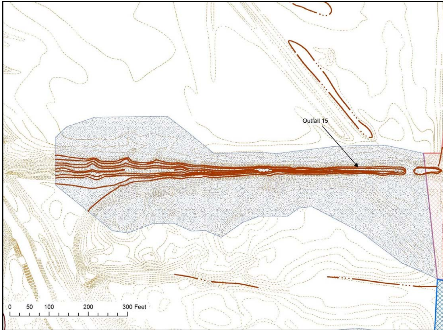
Figure 5. Proposed Embankment for Outfall 015 Pond
