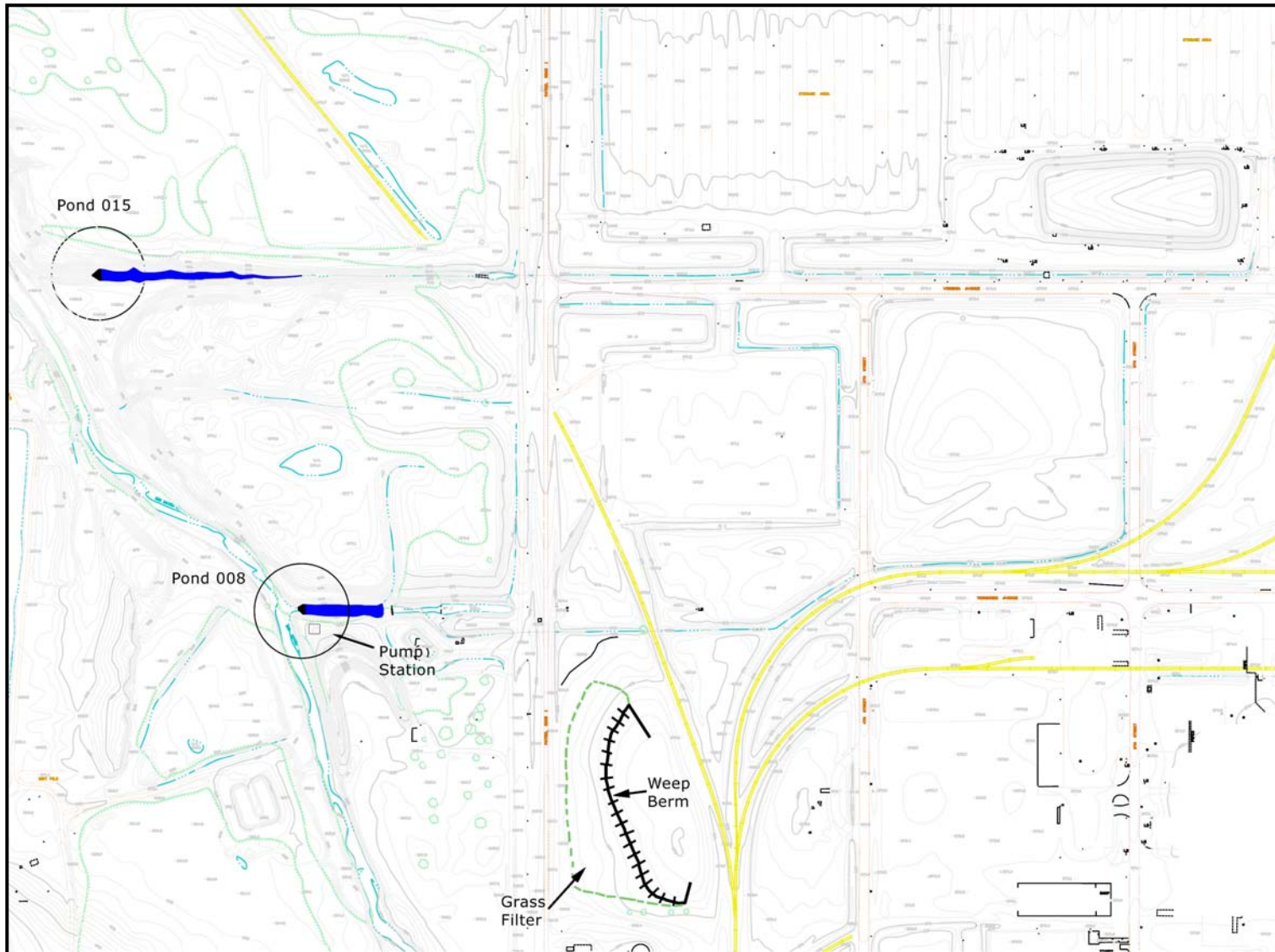
Figure 13. Overview of Outfall 008 Treatment System
