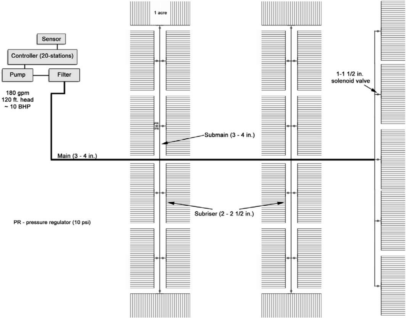
Figure 10. 25-Acre Drip and Micro-sprinkler Irrigation System Layout
