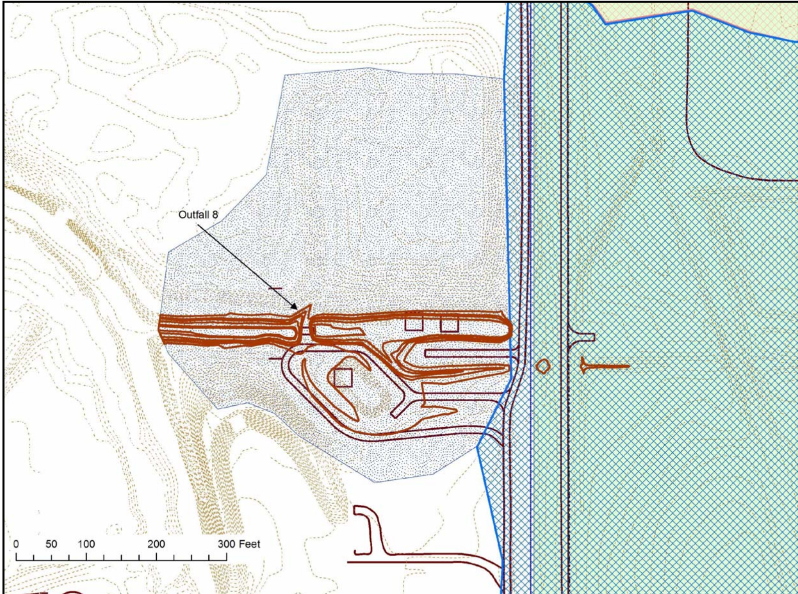
Figure 6. Proposed Embankment for Outfall 008 Pond
